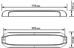
The dimensions are including the bezel. Dimensions of warning light only (WxHxD): 100x23x10mm
